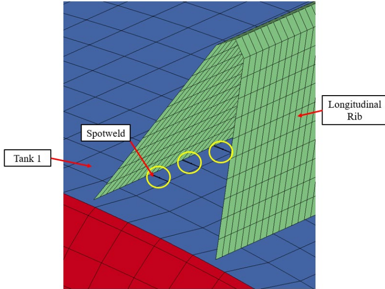
Figure 3.7 Spotweld Constraint
