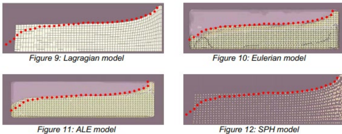
Figure 2.15 Fluid Model Comparison [9]
