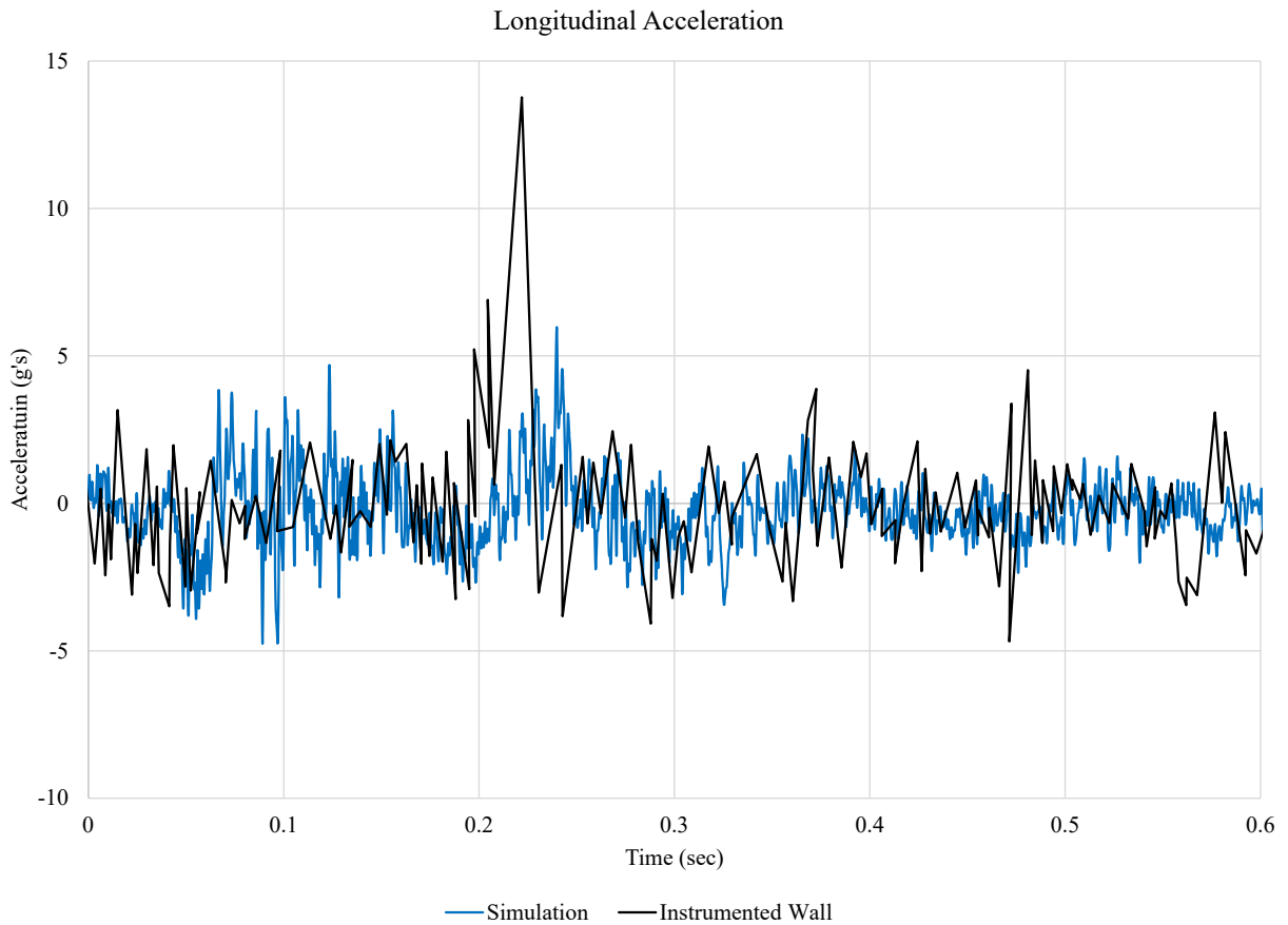
Figure 5.6 Longitudinal Acceleration
