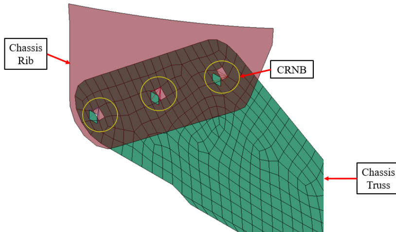
Figure 3.8 CRNB Constraint
