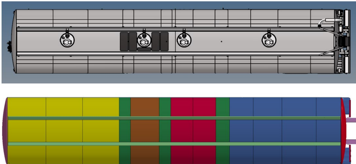
Figure 3.22 LBT Inc. Trailer Model Top View (Top) and LS-DYNA Model Top View (Bottom)
