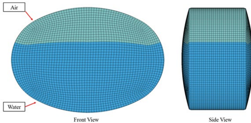
Figure 4.11 ALE Fluid Components
