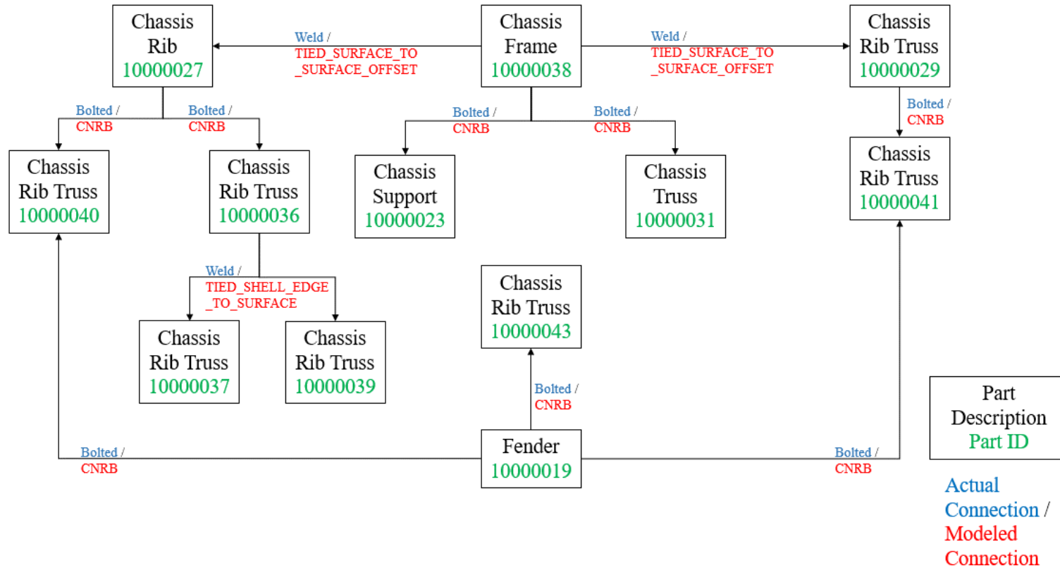
Figure B.3 Chassis Connection Diagram
